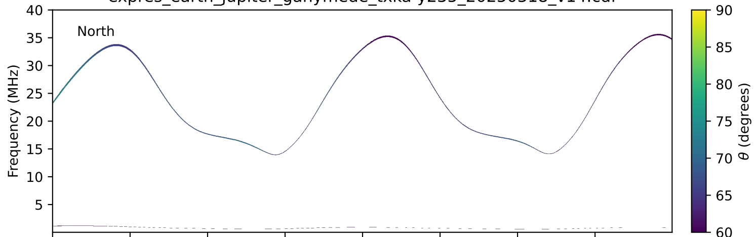
expres_earth_jupiter_ganymede_txka-y235_20250318_v14.cdf
