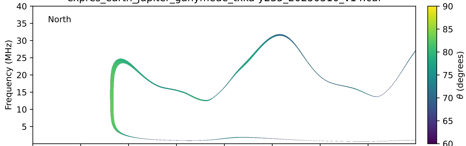
expres_earth_jupiter_ganymede_txka-y235_20250310_v14.cdf
