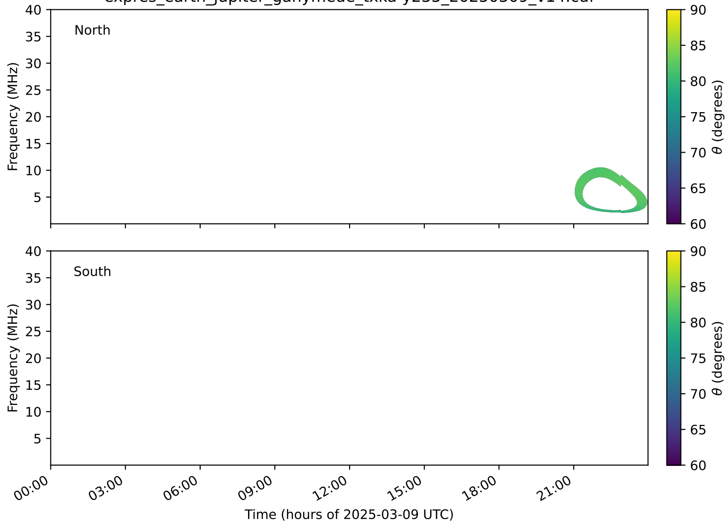
expres_earth_jupiter_ganymede_txka-y235_20250309_v14.cdf
