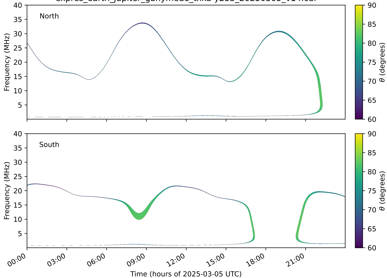
expres_earth_jupiter_ganymede_txka-y235_20250305_v14.cdf
