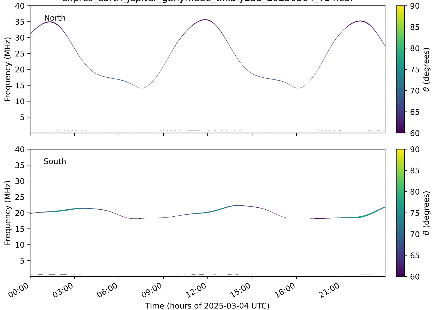
expres_earth_jupiter_ganymede_txka-y235_20250304_v14.cdf
