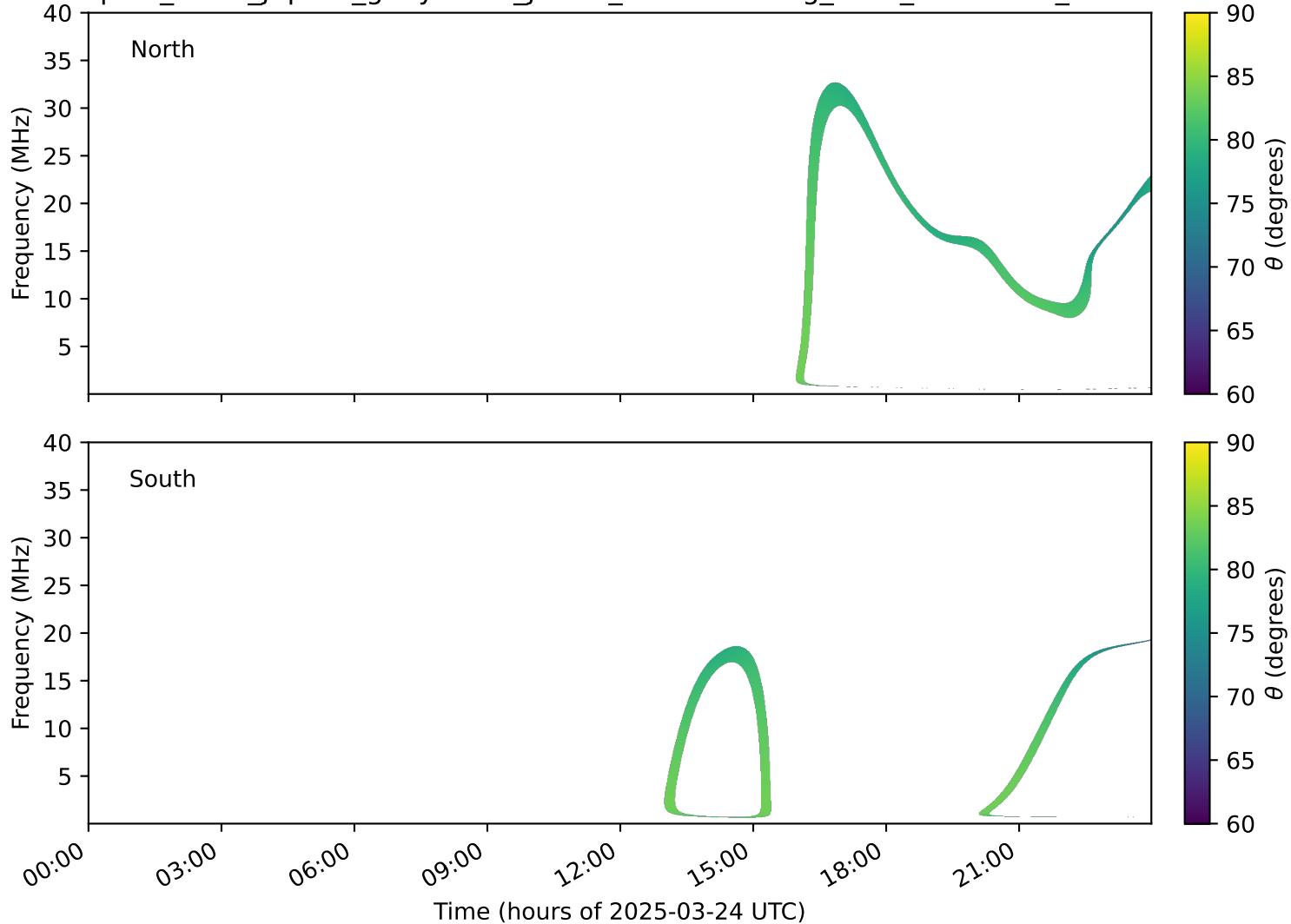
expres_earth_jupiter_ganymede_jrm33_lossc-wid1deg_3kev_20250324_v11.cdf
