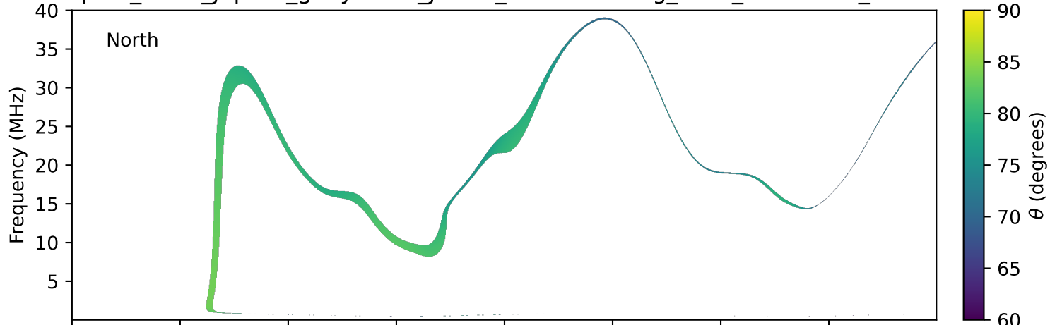
expres_earth_jupiter_ganymede_jrm33_lossc-wid1deg_3kev_20250303_v11.cdf
