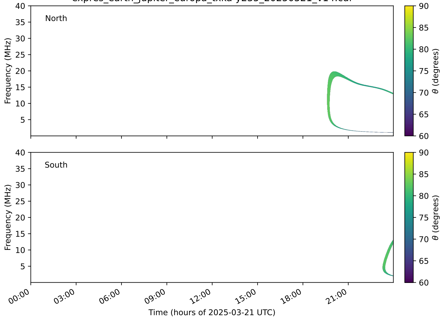
expres_earth_jupiter_europa_txka-y235_20250321_v14.cdf
