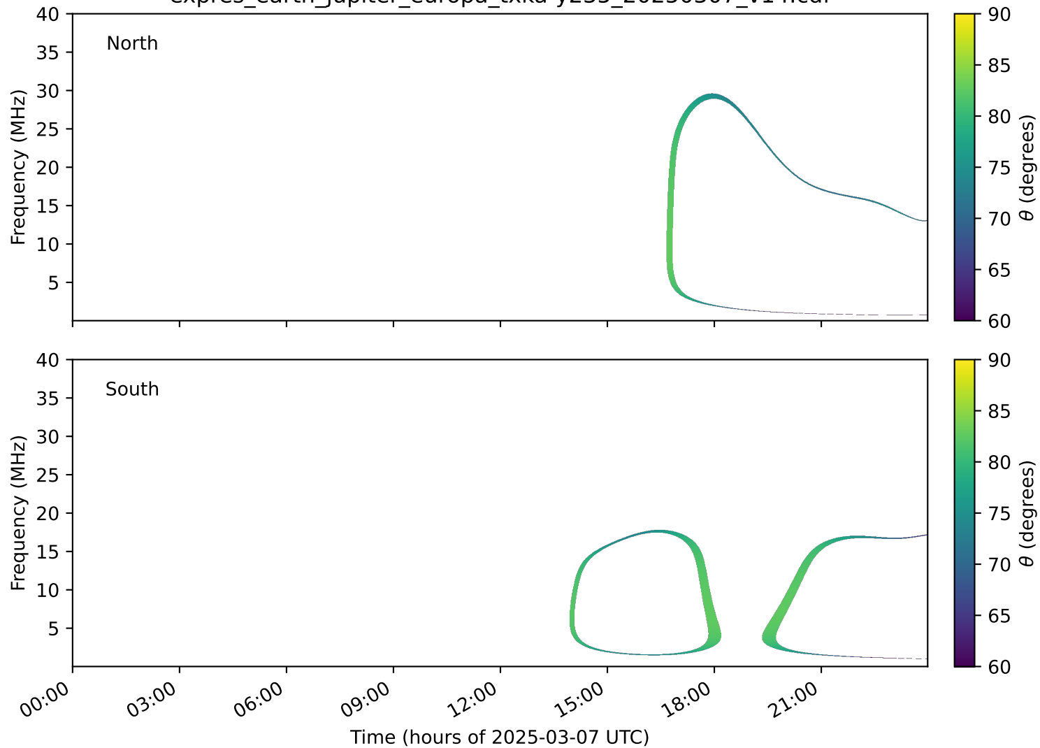
expres_earth_jupiter_europa_txka-y235_20250307_v14.cdf
