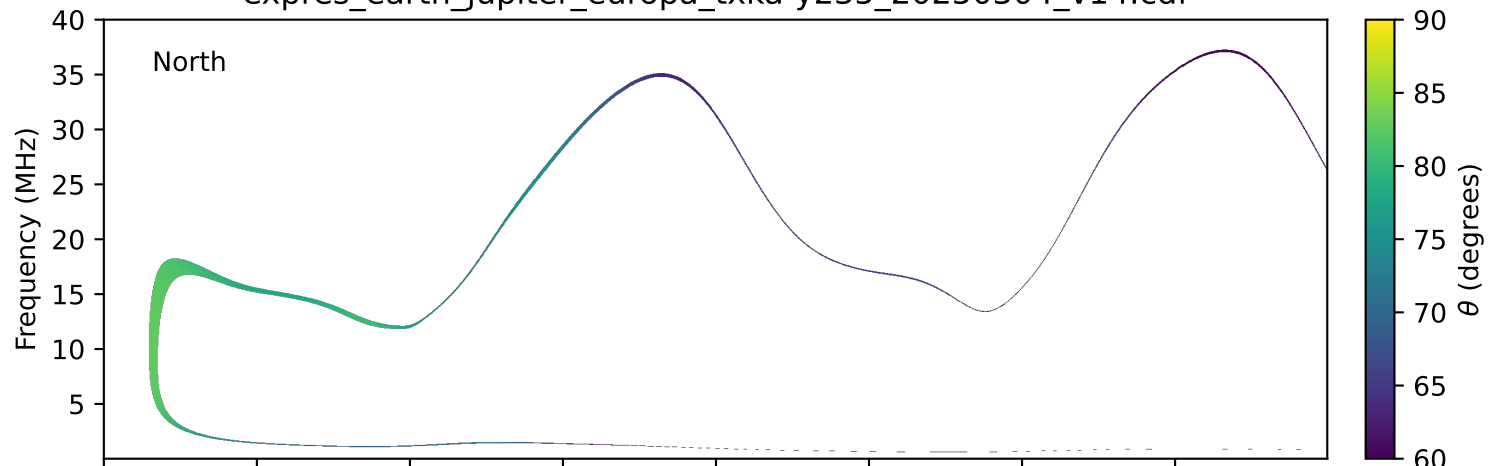
expres_earth_jupiter_europa_txka-y235_20250304_v14.cdf
