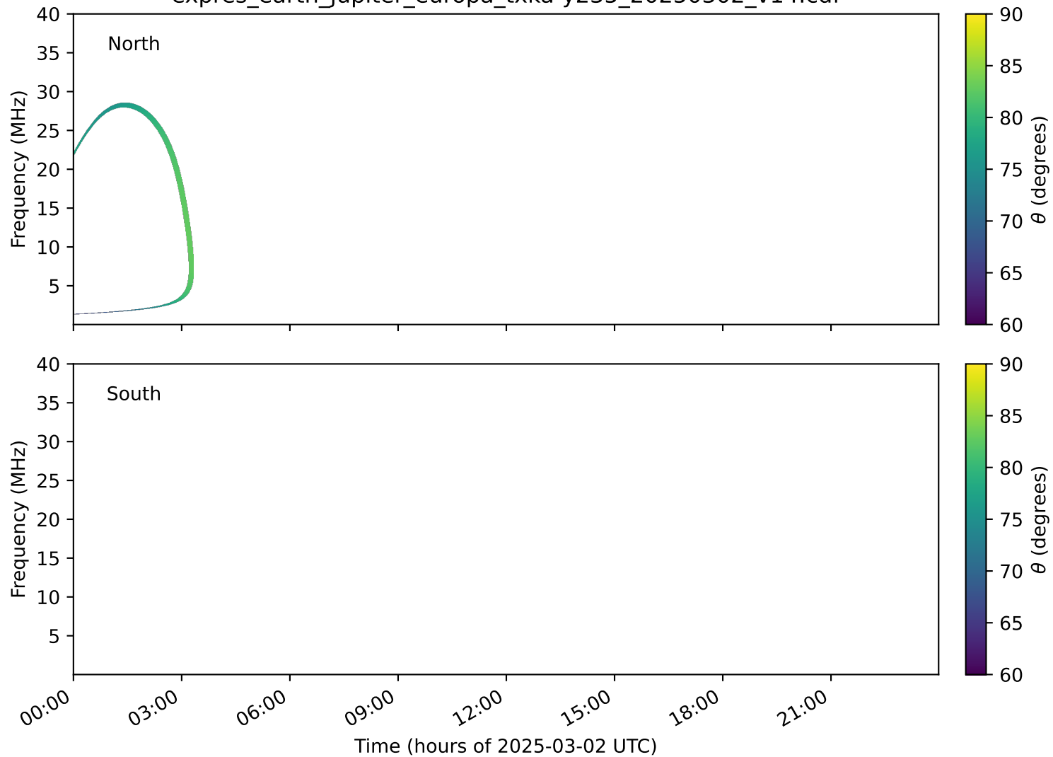
expres_earth_jupiter_europa_txka-y235_20250302_v14.cdf
