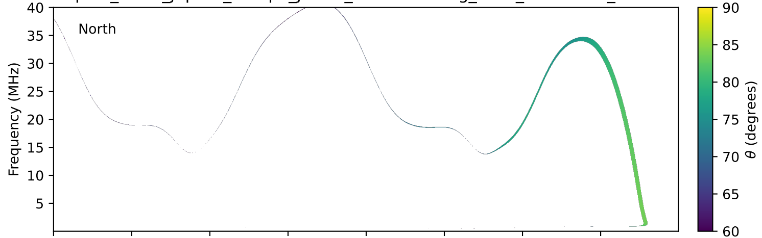
expres_earth_jupiter_europa_jrm33_lossc-wid1deg_3kev_20250319_v11.cdf
