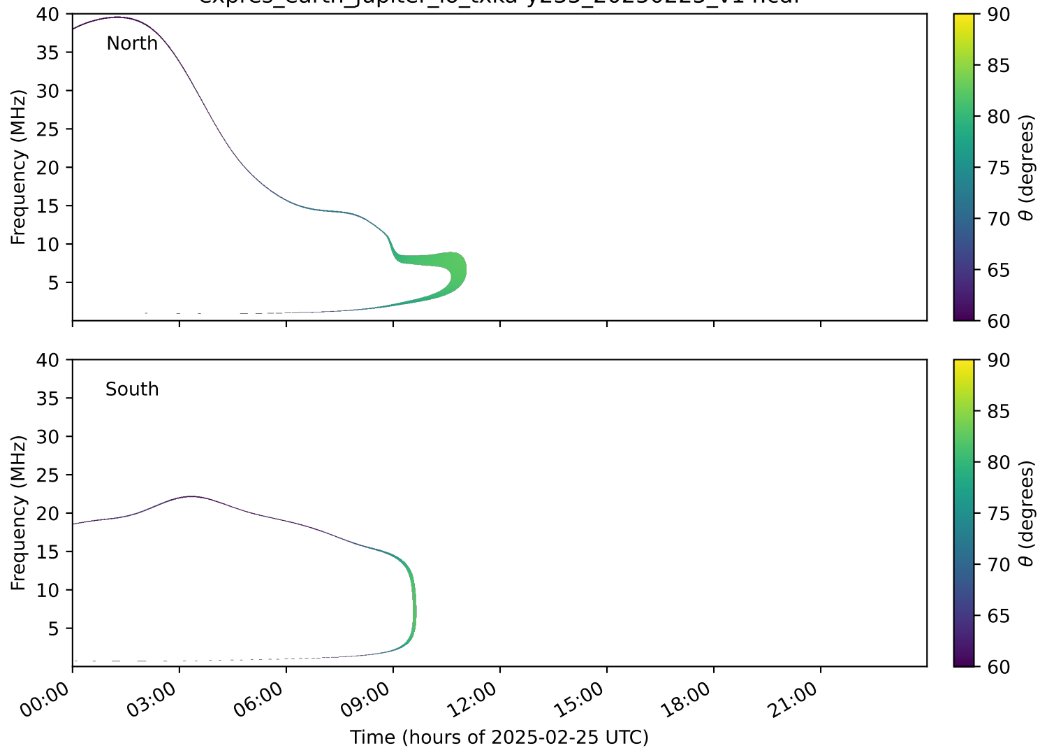
expres_earth_jupiter_io_txka-y235_20250225_v14.cdf
