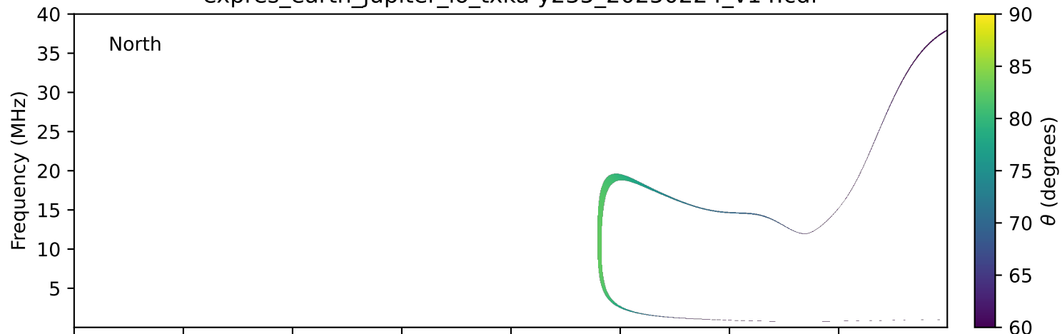
expres_earth_jupiter_io_txka-y235_20250224_v14.cdf
