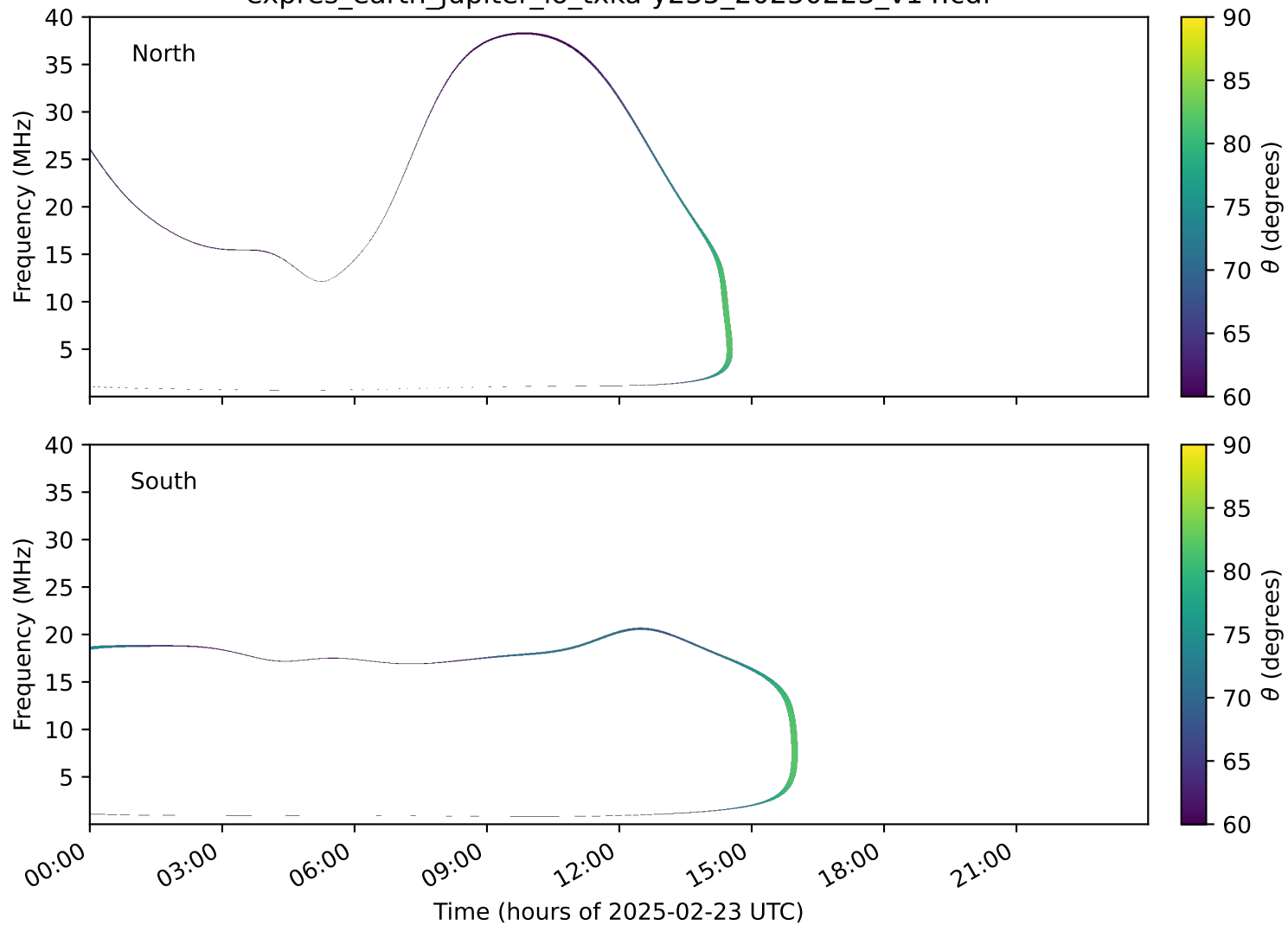
expres_earth_jupiter_io_txka-y235_20250223_v14.cdf
