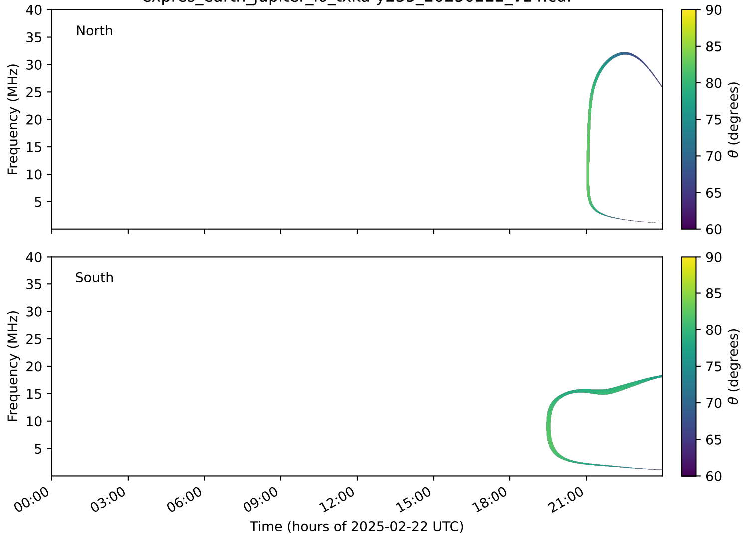
expres_earth_jupiter_io_txka-y235_20250222_v14.cdf
