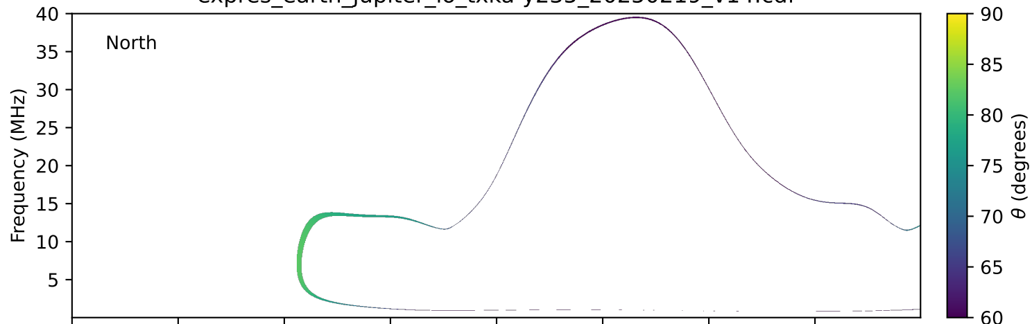
expres_earth_jupiter_io_txka-y235_20250219_v14.cdf
