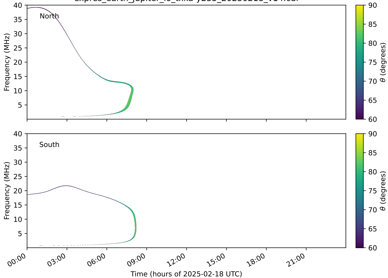
expres_earth_jupiter_io_txka-y235_20250218_v14.cdf
