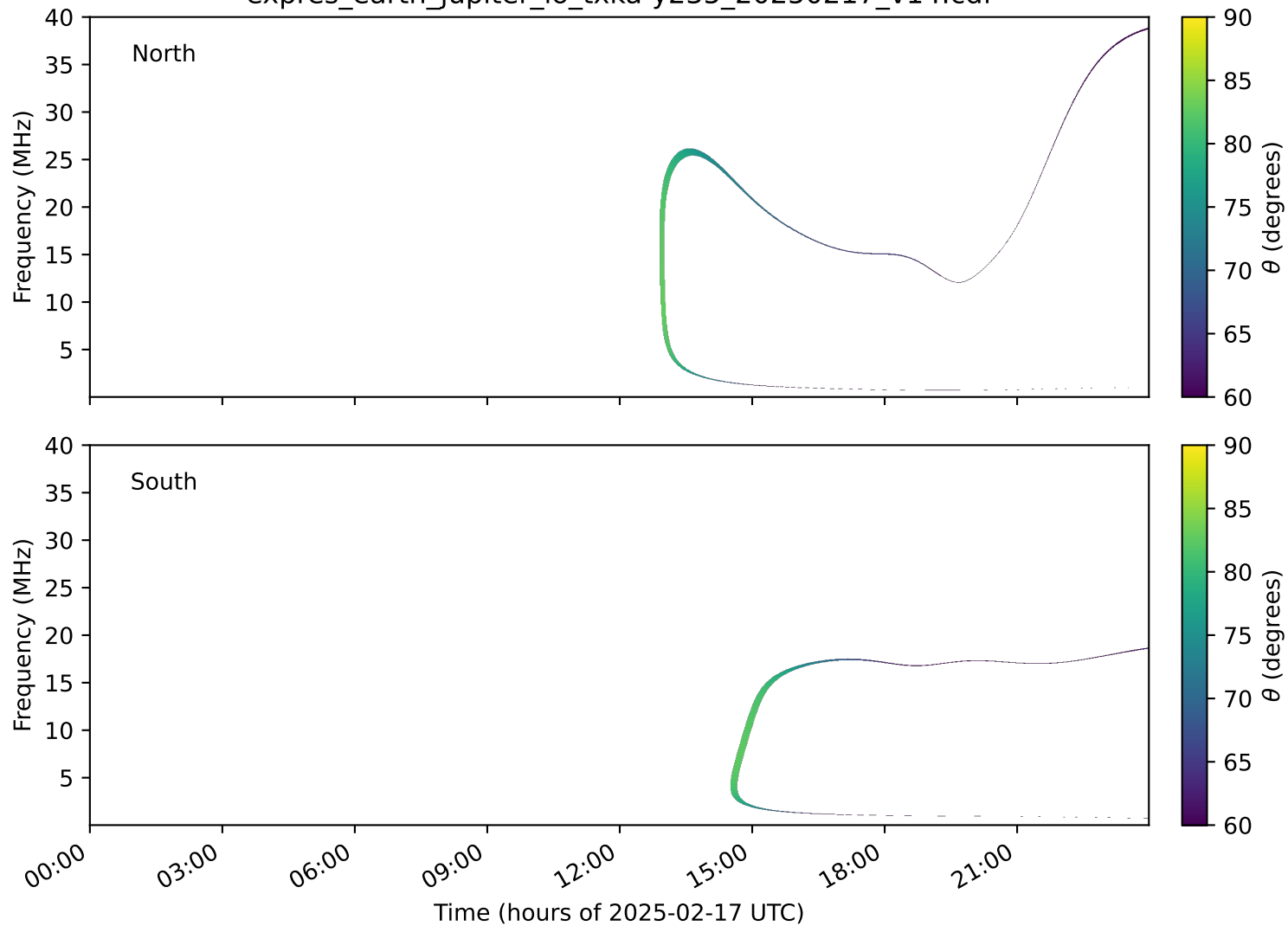
expres_earth_jupiter_io_txka-y235_20250217_v14.cdf
