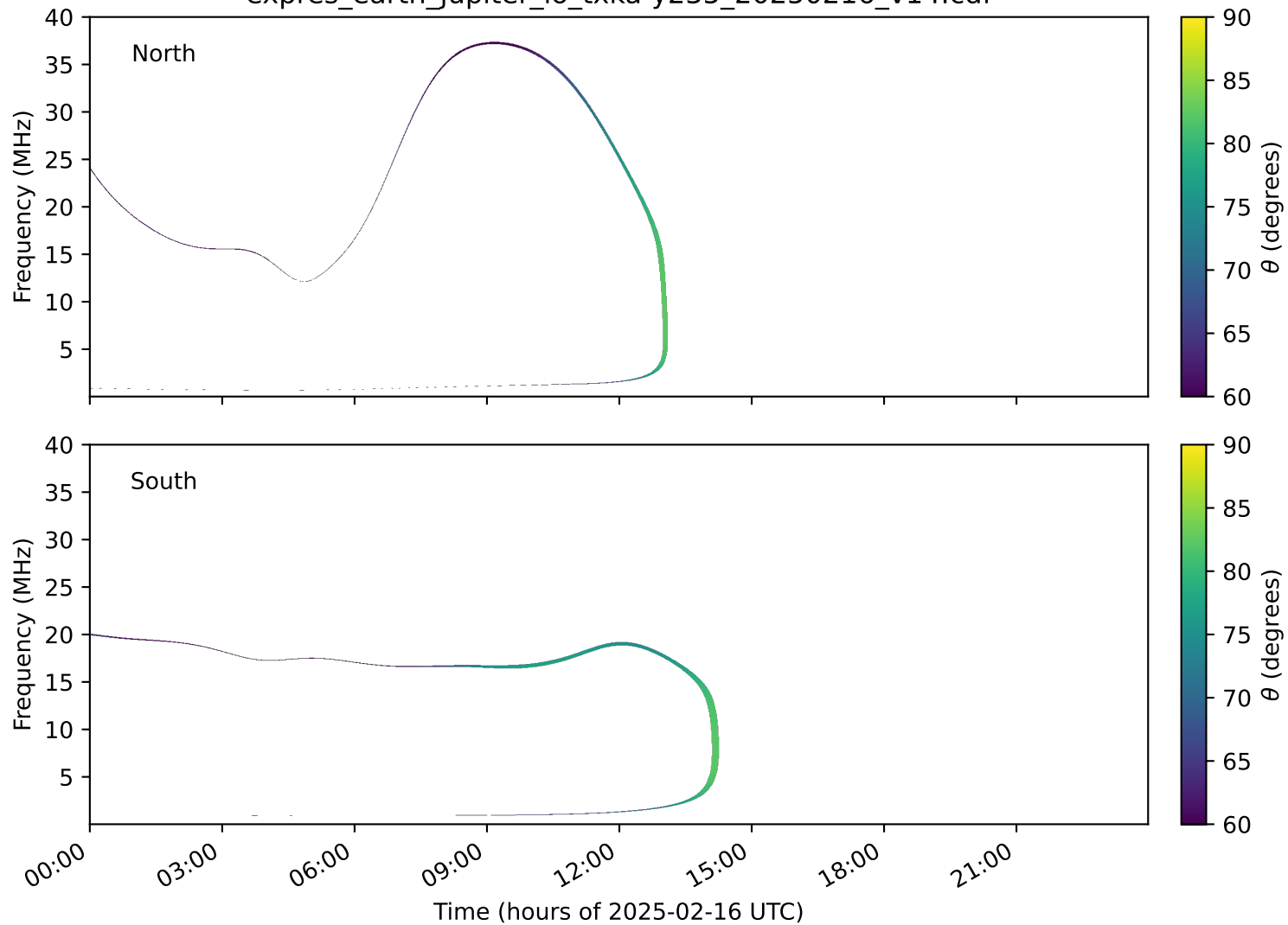
expres_earth_jupiter_io_txka-y235_20250216_v14.cdf
