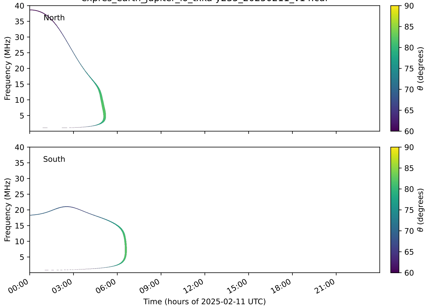
expres_earth_jupiter_io_txka-y235_20250211_v14.cdf
