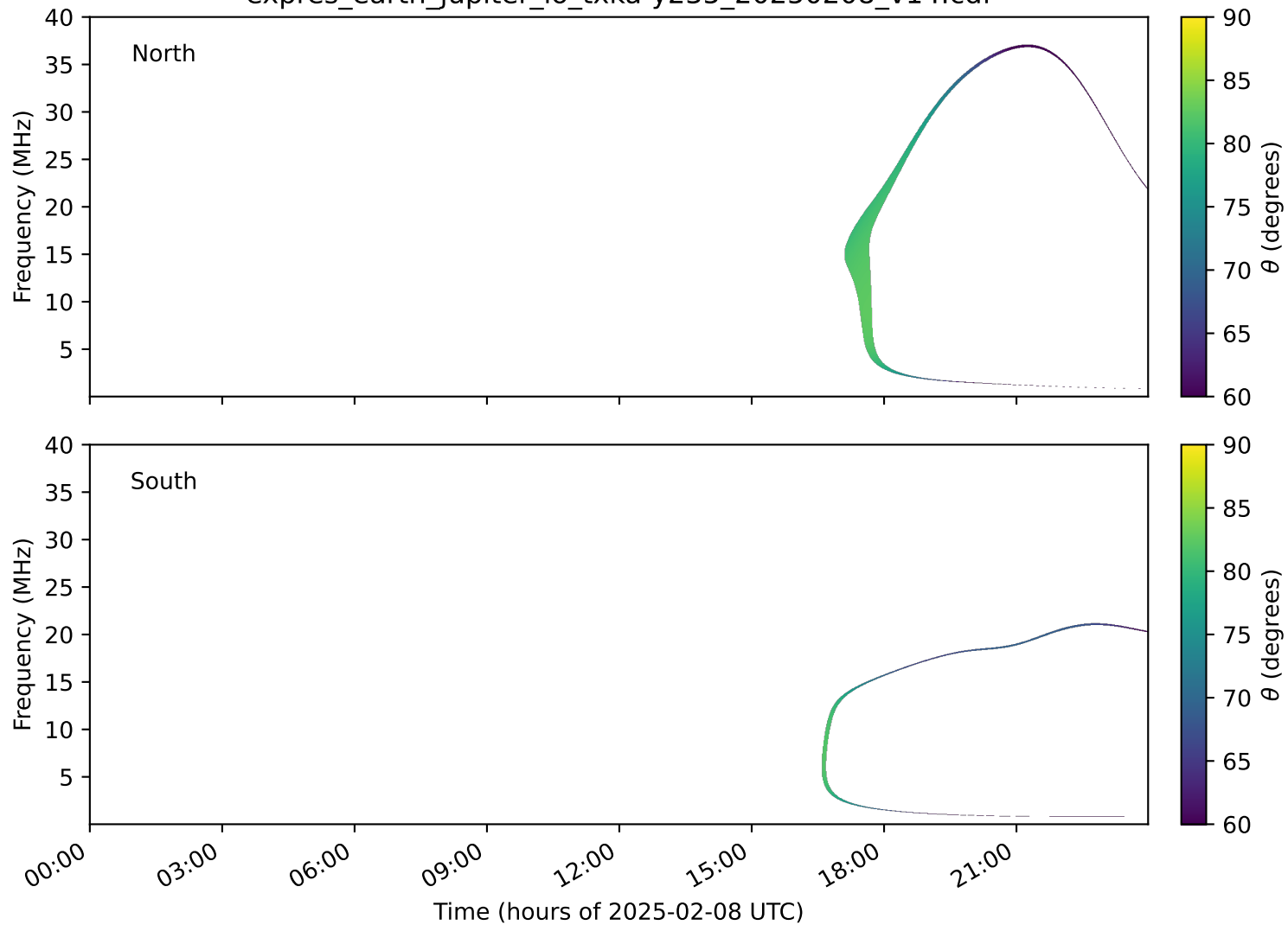
expres_earth_jupiter_io_txka-y235_20250208_v14.cdf
