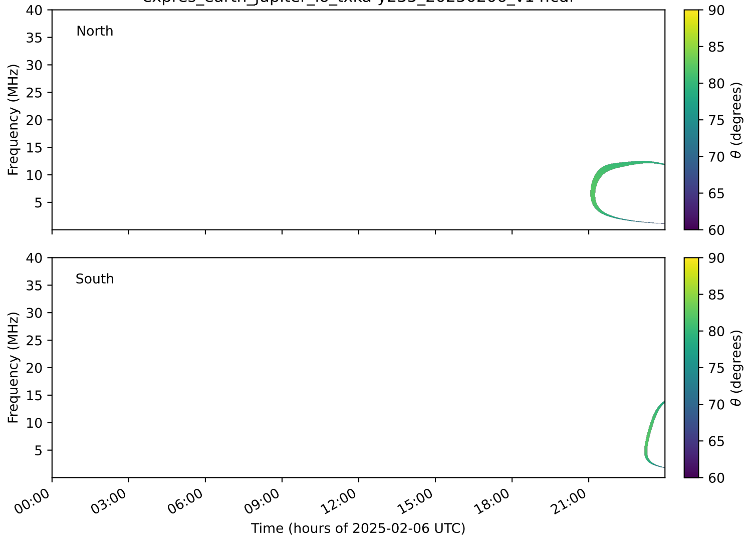
expres_earth_jupiter_io_txka-y235_20250206_v14.cdf
