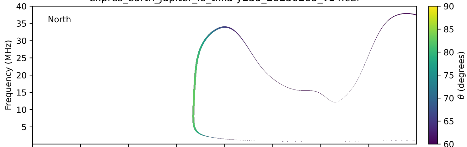
expres_earth_jupiter_io_txka-y235_20250203_v14.cdf
