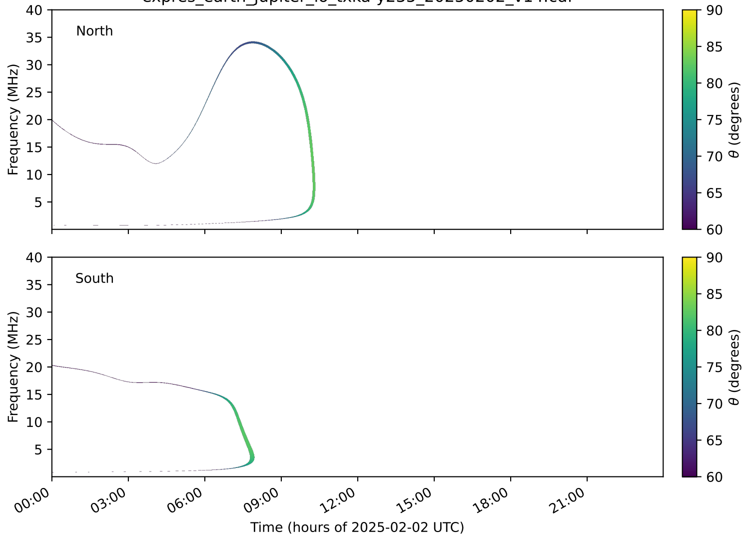
expres_earth_jupiter_io_txka-y235_20250202_v14.cdf
