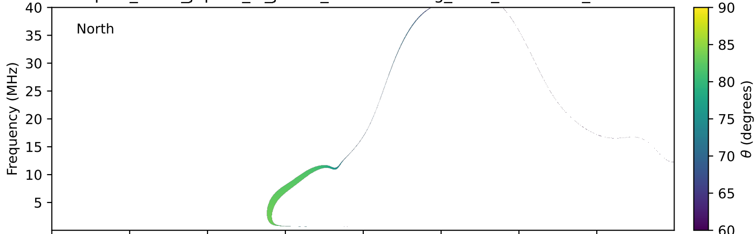
expres_earth_jupiter_io_jrm33_lossc-wid1deg_3kev_20250226_v11.cdf
