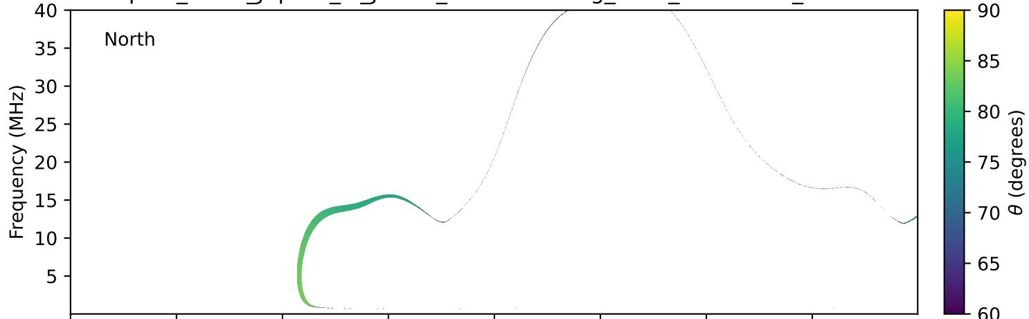
expres_earth_jupiter_io_jrm33_lossc-wid1deg_3kev_20250219_v11.cdf
