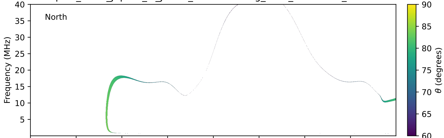
expres_earth_jupiter_io_jrm33_lossc-wid1deg_3kev_20250212_v11.cdf
