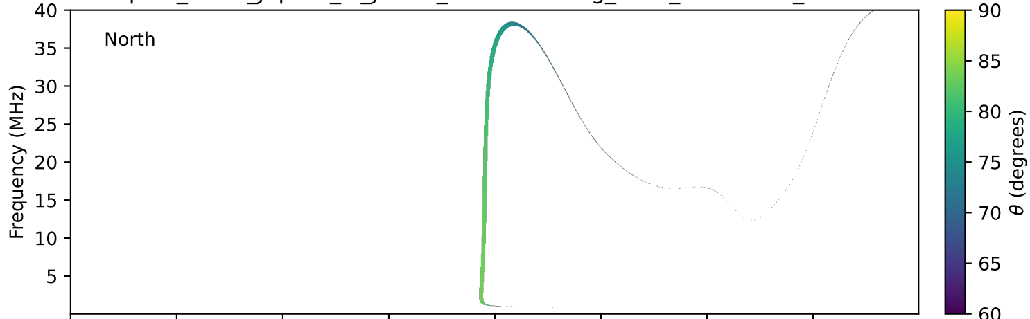
expres_earth_jupiter_io_jrm33_lossc-wid1deg_3kev_20250210_v11.cdf
