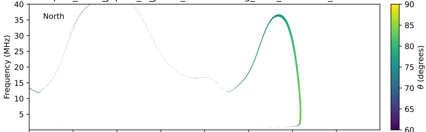
expres_earth_jupiter_io_jrm33_lossc-wid1deg_3kev_20250207_v11.cdf
