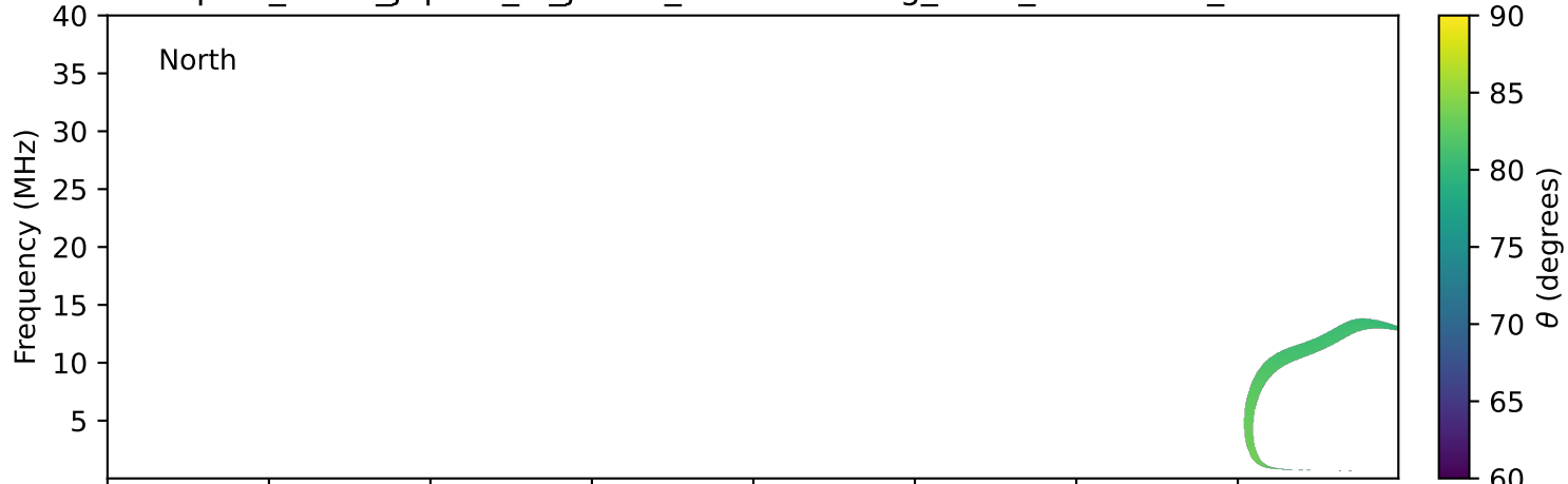
expres_earth_jupiter_io_jrm33_lossc-wid1deg_3kev_20250206_v11.cdf
