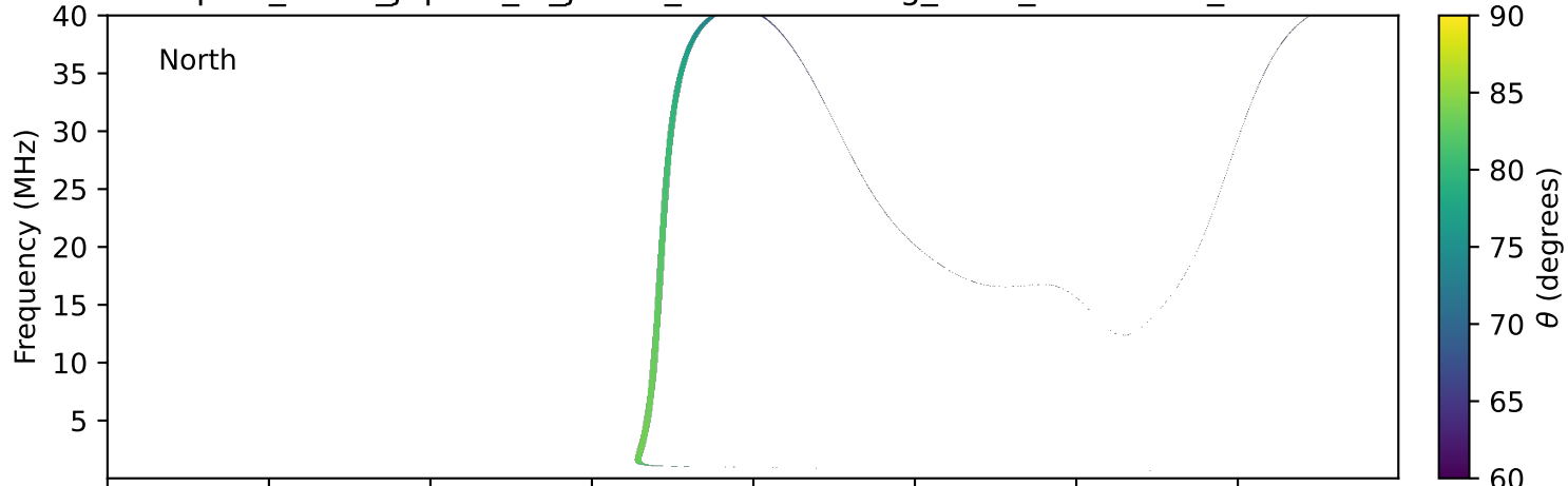
expres_earth_jupiter_io_jrm33_lossc-wid1deg_3kev_20250203_v11.cdf
