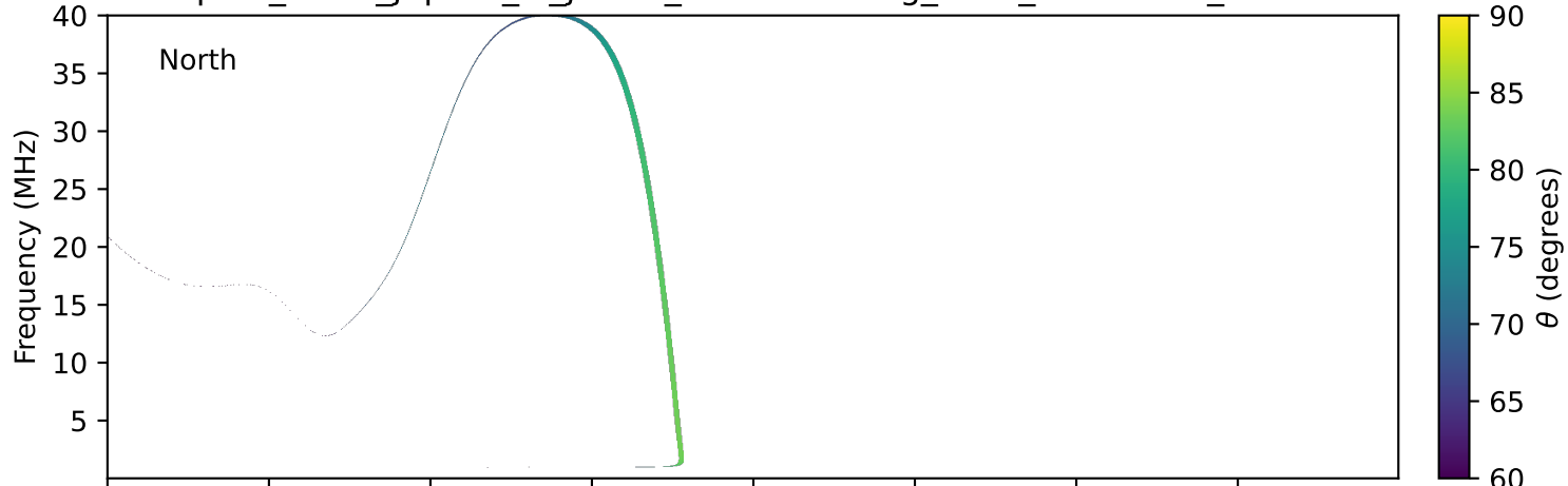
expres_earth_jupiter_io_jrm33_lossc-wid1deg_3kev_20250202_v11.cdf
