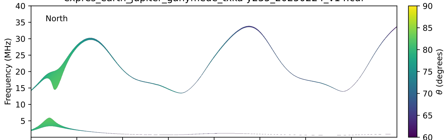
expres_earth_jupiter_ganymede_txka-y235_20250224_v14.cdf
