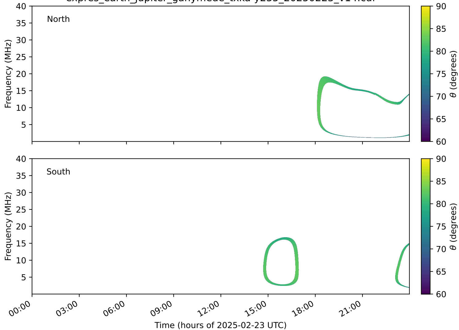
expres_earth_jupiter_ganymede_txka-y235_20250223_v14.cdf
