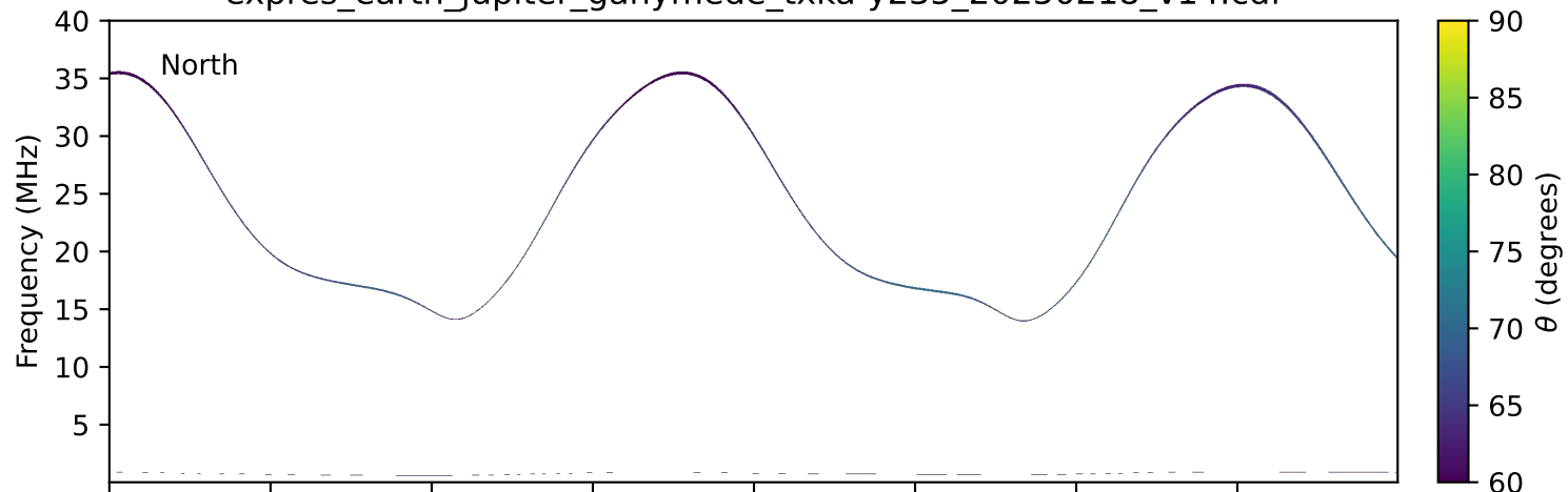
expres_earth_jupiter_ganymede_txka-y235_20250218_v14.cdf
