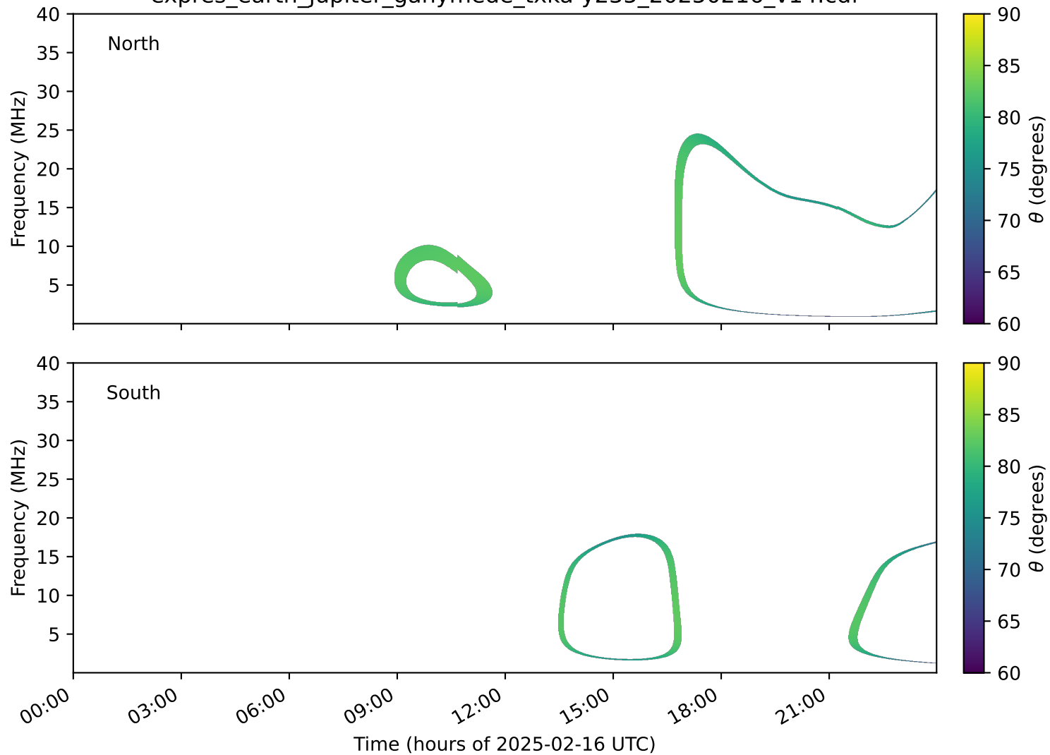
expres_earth_jupiter_ganymede_txka-y235_20250216_v14.cdf
