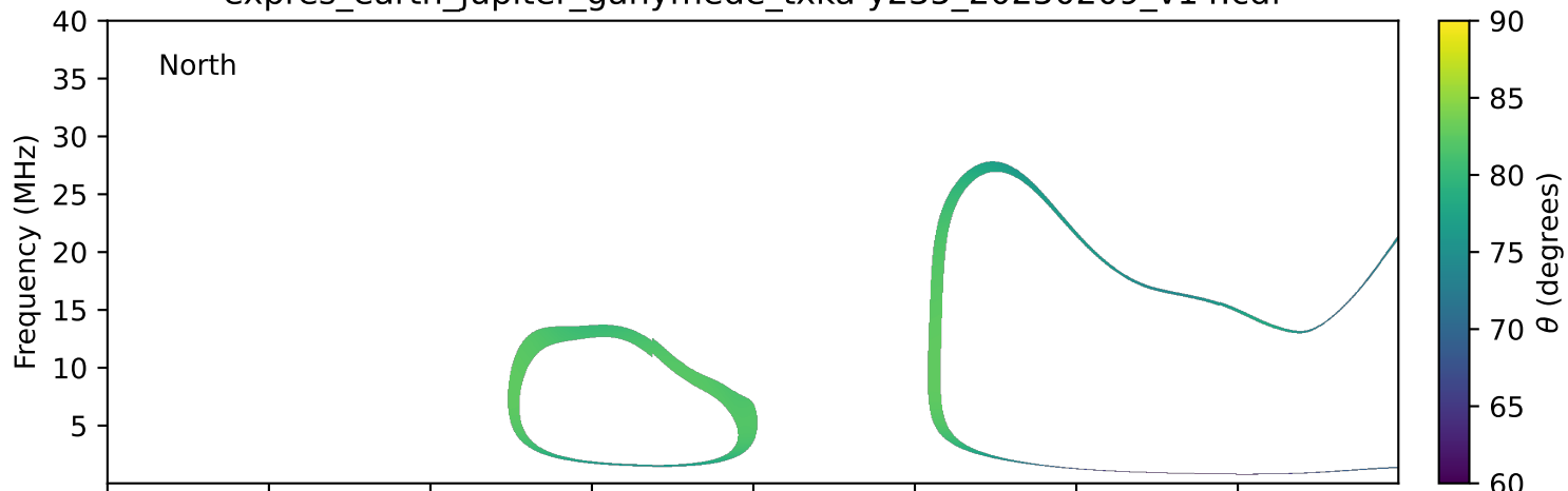
expres_earth_jupiter_ganymede_txka-y235_20250209_v14.cdf
