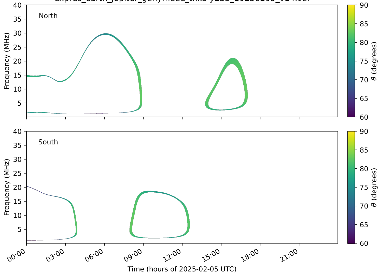
expres_earth_jupiter_ganymede_txka-y235_20250205_v14.cdf
