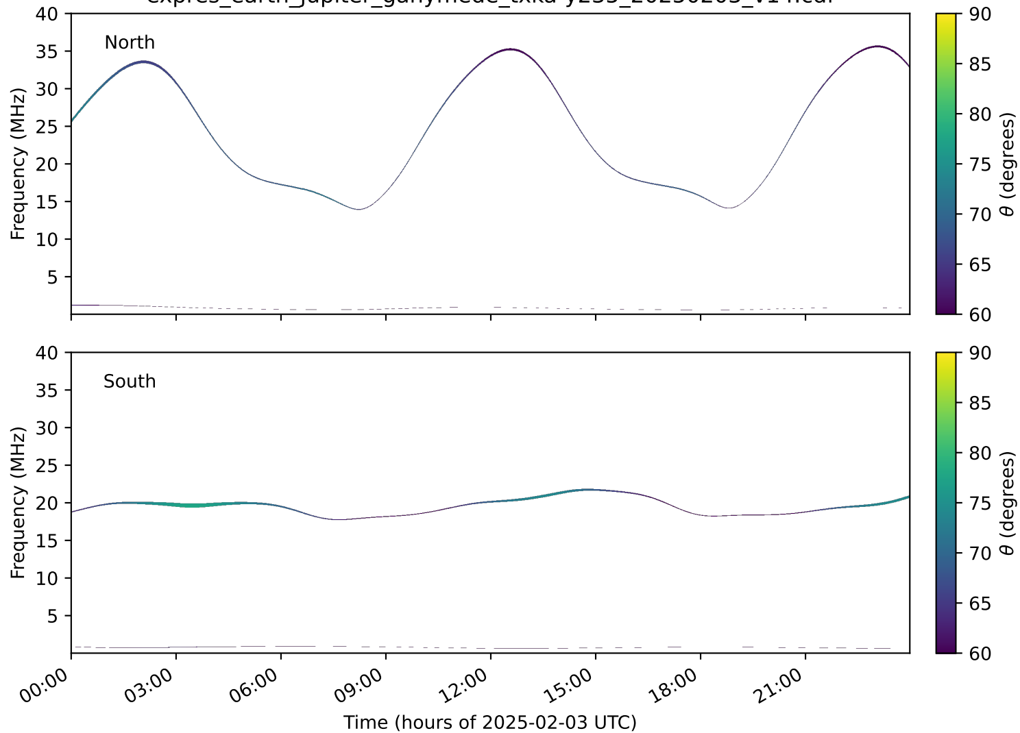
expres_earth_jupiter_ganymede_txka-y235_20250203_v14.cdf
