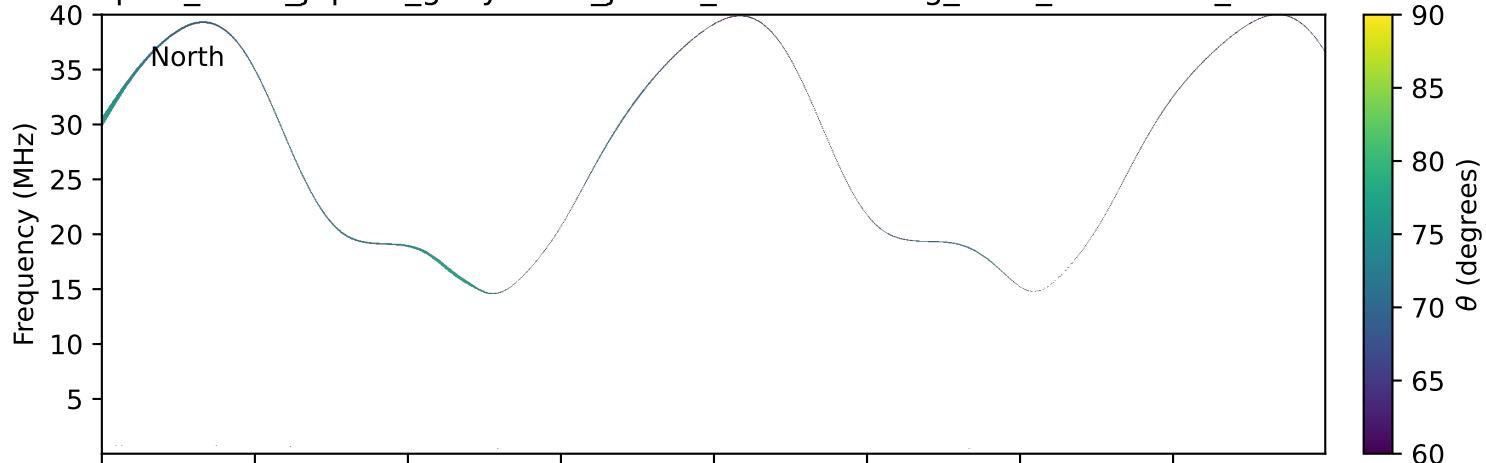
expres_earth_jupiter_ganymede_jrm33_lossc-wid1deg_3kev_20250203_v11.cdf
