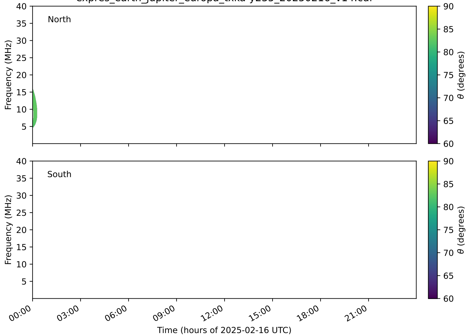
expres_earth_jupiter_europa_txka-y235_20250216_v14.cdf
