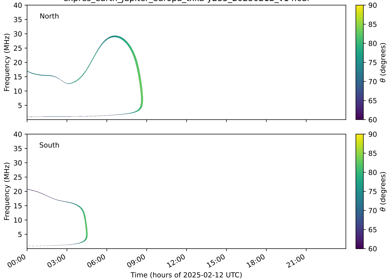
expres_earth_jupiter_europa_txka-y235_20250212_v14.cdf
