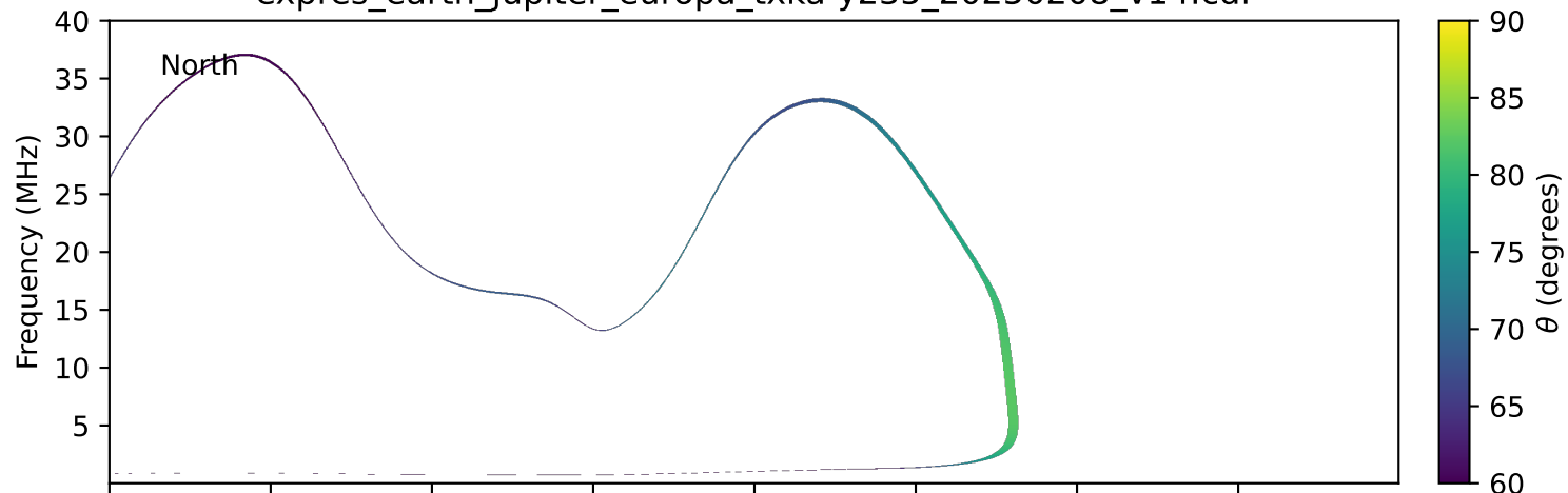
expres_earth_jupiter_europa_txka-y235_20250208_v14.cdf
