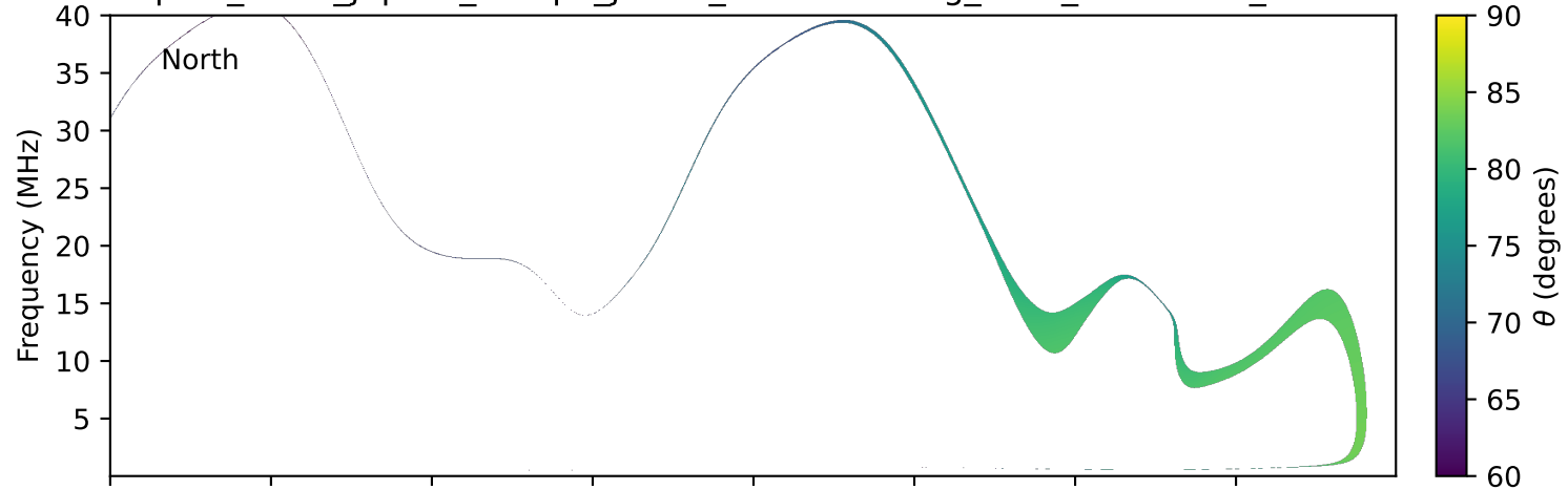
expres_earth_jupiter_europa_jrm33_lossc-wid1deg_3kev_20250208_v11.cdf
