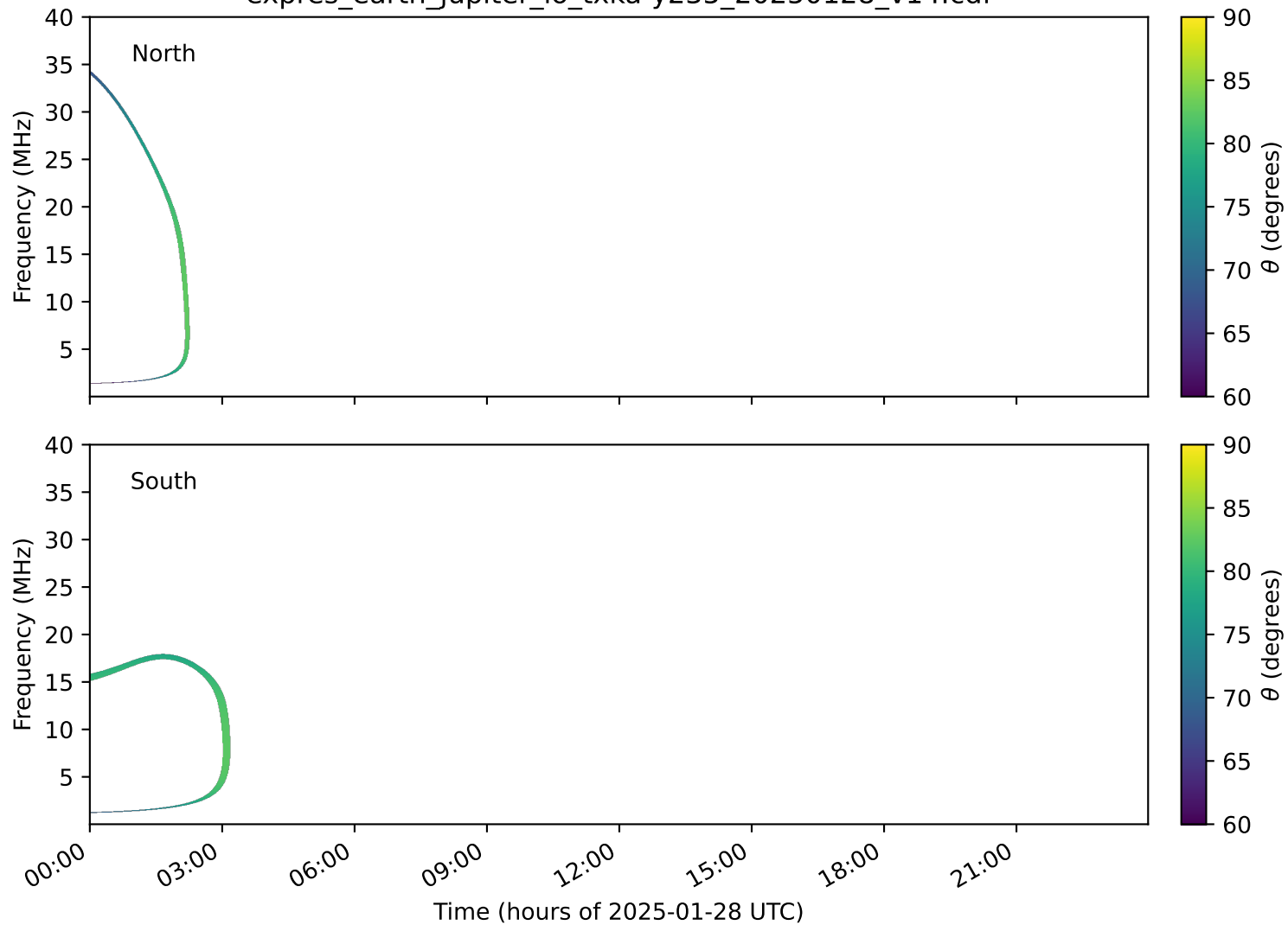
expres_earth_jupiter_io_txka-y235_20250128_v14.cdf
