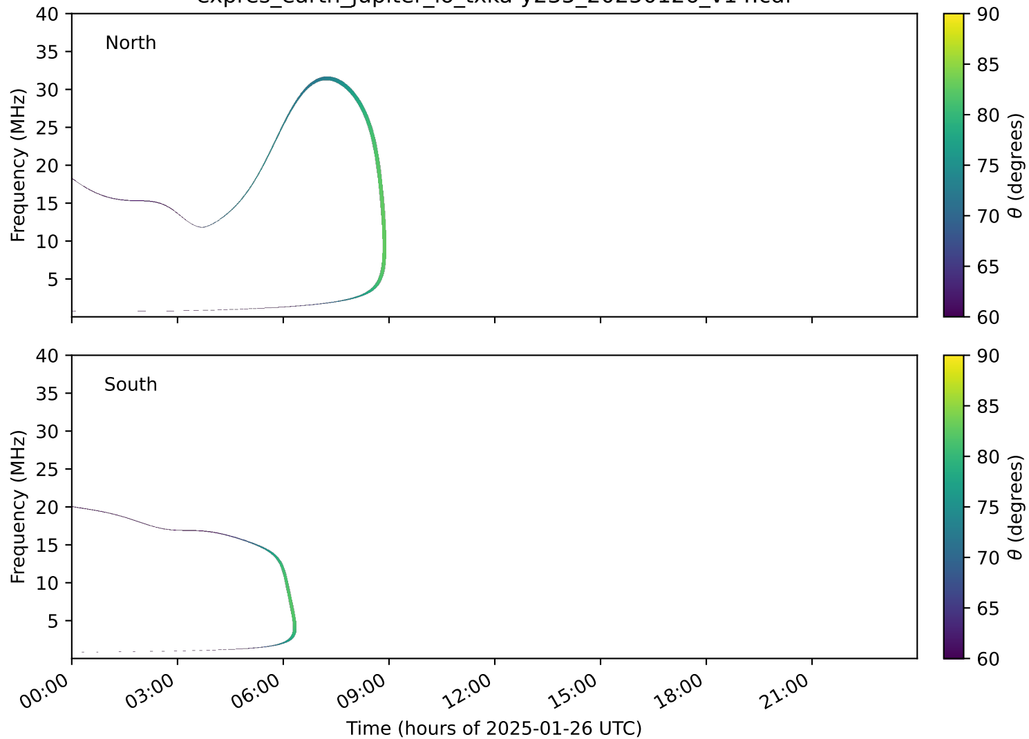
expres_earth_jupiter_io_txka-y235_20250126_v14.cdf
