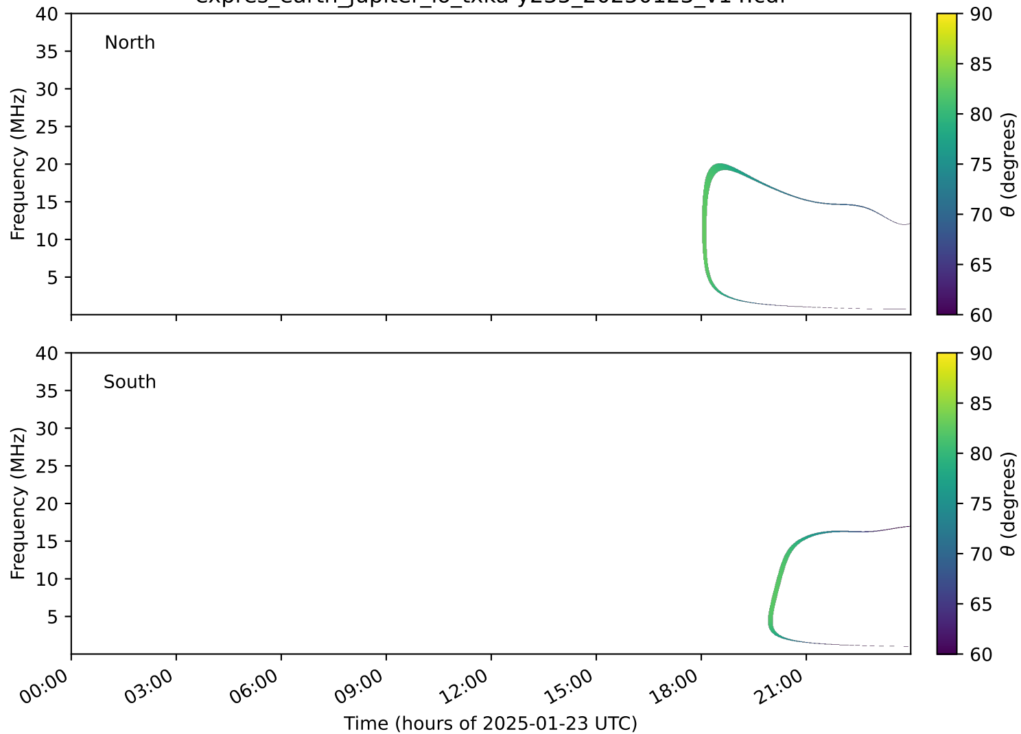
expres_earth_jupiter_io_txka-y235_20250123_v14.cdf
