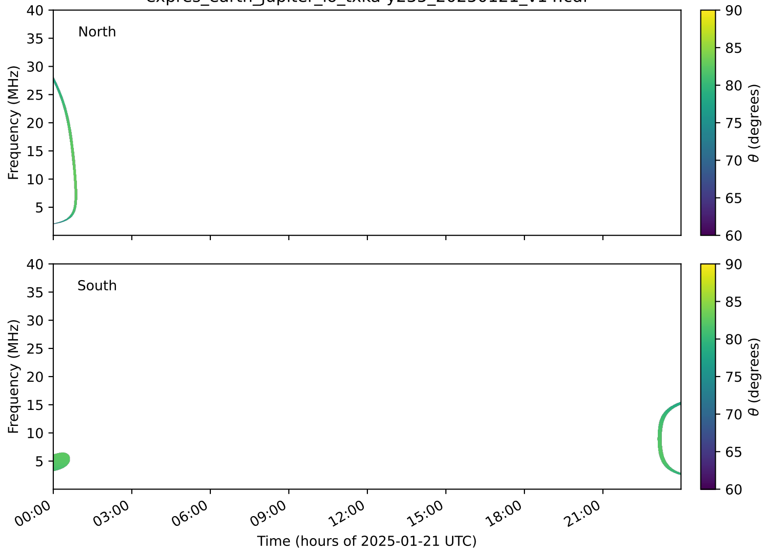
expres_earth_jupiter_io_txka-y235_20250121_v14.cdf
