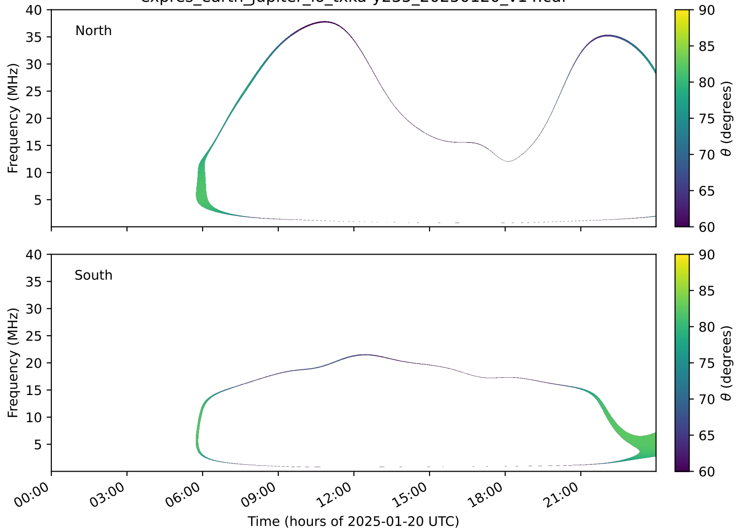
expres_earth_jupiter_io_txka-y235_20250120_v14.cdf
